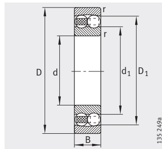
Cylindrical bore
