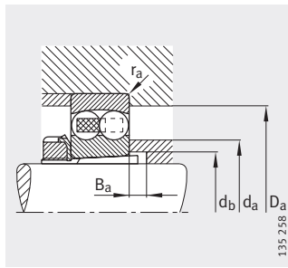
Mounting dimensions
