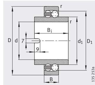
Extended inner ring
