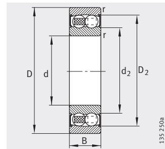
Cylindrical bore 2RS seals
