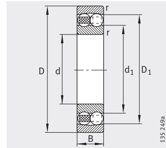
Cylindrical bore
