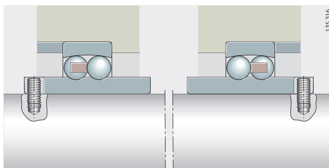
Figure 2 Location and arrangement of bearings
