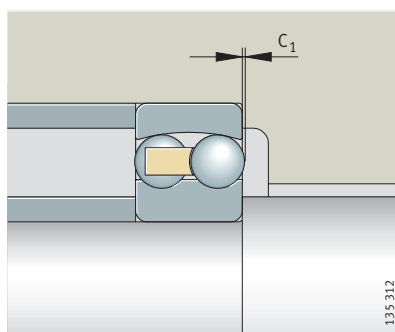
Figure 1 Ball projection C_1
