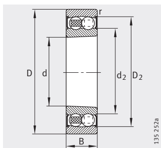
Tapered bore K = taper 1:12 2RS seals
