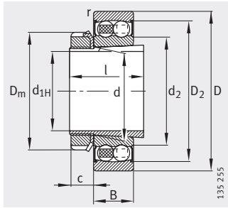
2RS seals
